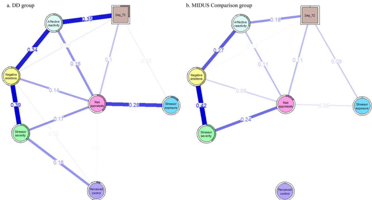
Figure 2. Network graphs of daily stress process components and depressive symptoms at Time 2 by group. Edge thickness represents the strength of associations, with blue edges indicating positive associations. The colored segments of the rings around each node indicate the proportion of variance explained by all other nodes in the network.
