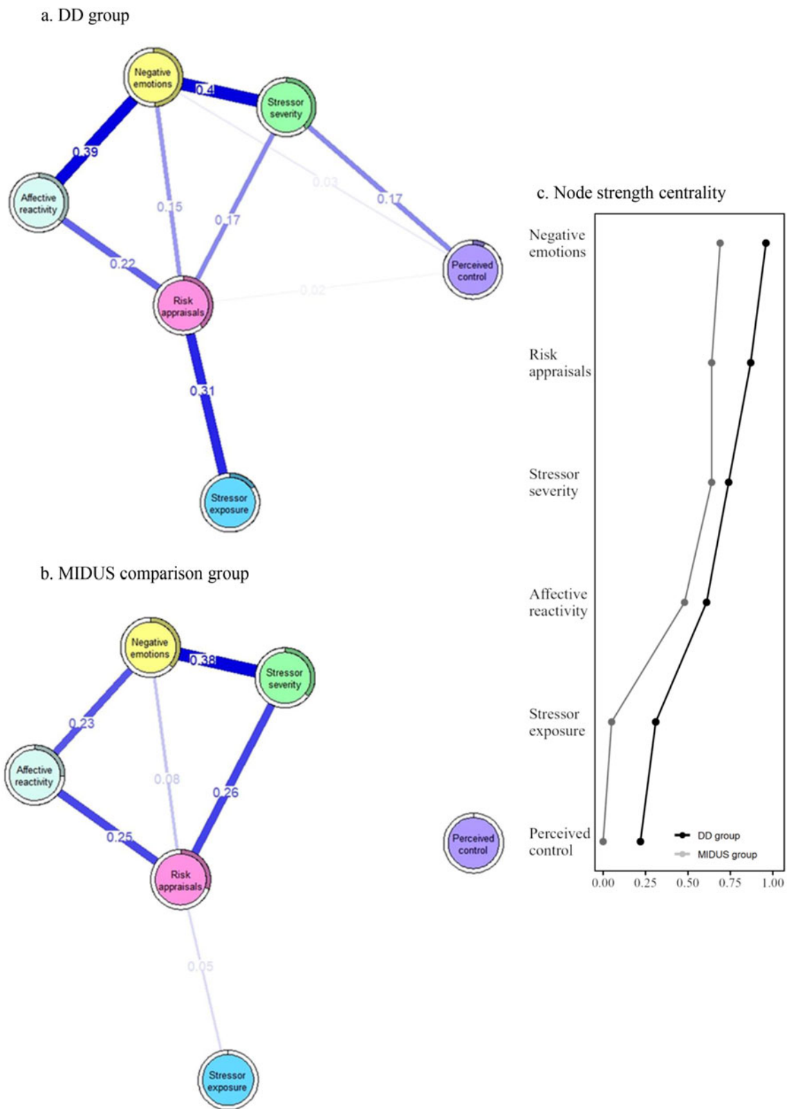
Figure 1. Regularized network graphs and node strength centrality of daily stress by group. (a) Network graph for the DD group; (b). Network graph for the MIDUS comparison group. In both panels (a). and (b). edge thickness represents the strength of associations, with blue edges indicating positive associations, and the colored segments of the rings around each node indicate the proportion of variance explained by all other nodes in the network. To ensure consistency, the same average layout was applied to both networks. (c). Node strength centrality of the daily stress networks for the DD and MIDUS comparison groups. The x-axis represents the z-standardized strength centrality values, and the y-axis indicates the daily stress processes.
